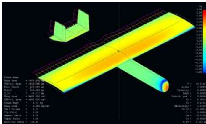
Fig.8 Analysis on Rectangular wing
