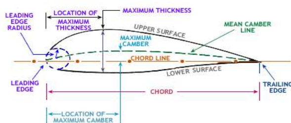
Fig.2 Airfoil nomenclature
