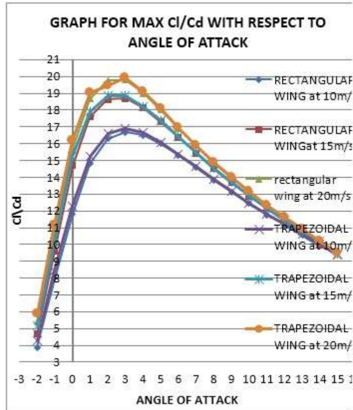
Fig.10 Graph of comparison between two wing's
