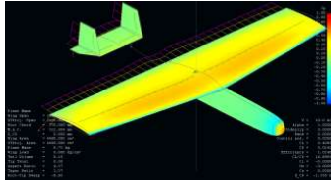
Fig.9 Analysis on Trapezoidal body
